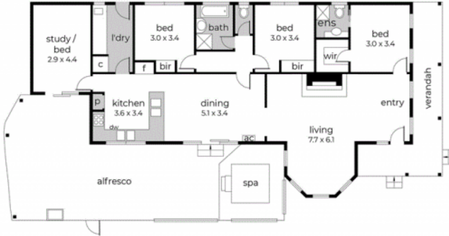
FLOOR PLAN
